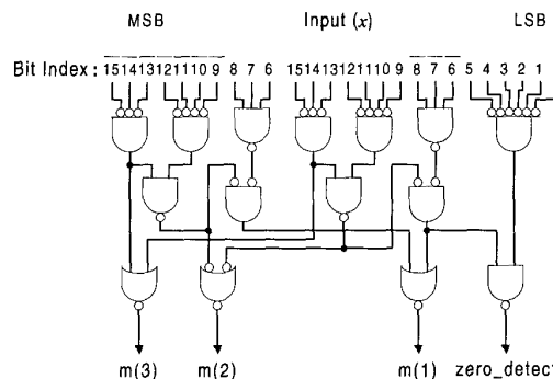
Figure 3. Mask and zero detection signals generation unit based on static logic.
