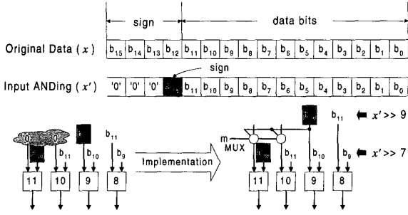
Figure 5. Example of the proposed mechanism for sign bit extension in the multiplier array.
