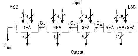
Figure 6. Static fine-grain partitioned adder architecture.
