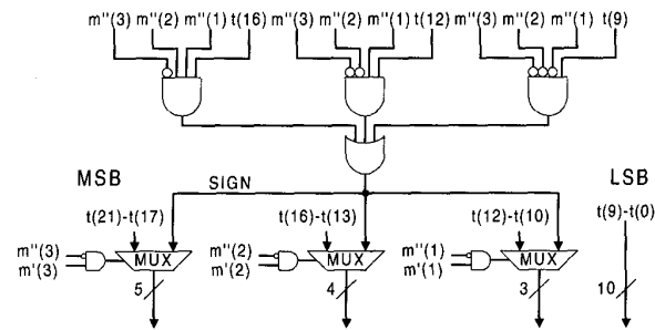
Figure 8. Partial sign bit recovery logic.
