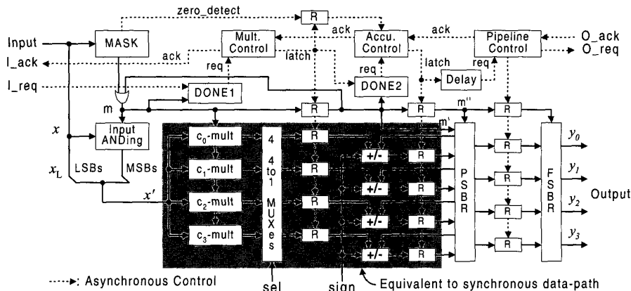
Figure 2. Proposed asynchronous 4x4 matrix-vector multiplier architecture.
