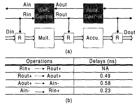
Figure 9. Adoption of 4-phase handshaking control scheme by Day and Woods; (a) pipeline stages and (b) control overhead analysis.
