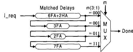
Figure 7. Speculative completion sensing using mask signals instead of abort logic.
